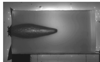
Whakaahua 4.17. .308W 165gr Koi Ngāwari (SP) projectile . Mauī: I mua i te pānga o te matā; Waenga: Pakarutanga tuatahi; Matau: Pakarutanga mutunga.
